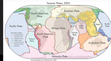
Tectonic map of the Earth. HAYSTOCK ET AL. 2022/EARTH-SCI. REV.
